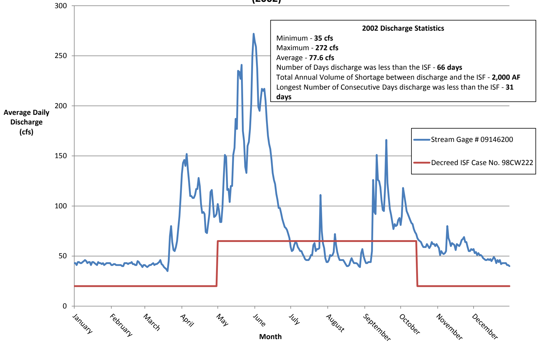
Figure 4 Uncompahgre River Streamflow and ISF Hydrograph (2002)
